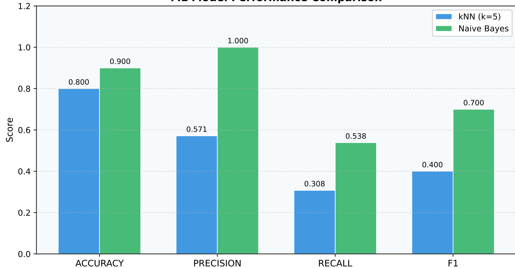
ML Model Performance Comparison
